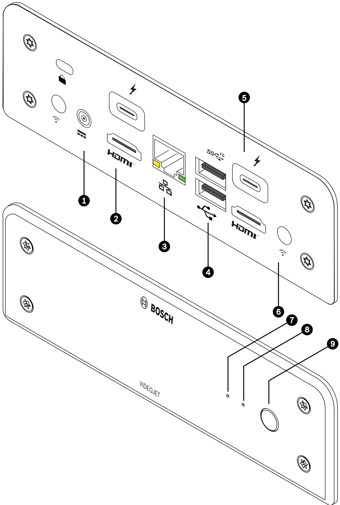
Figure 3.1: Connections, controls and displays
