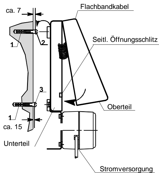
Abb. 6 Wandmontage Tenotime 2
