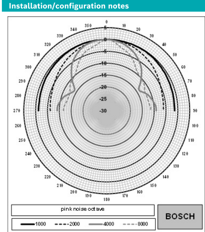
Fig. 1: Polar diagram LC1-PC30G6-6-IN high frequency part (frequency in Hz)
