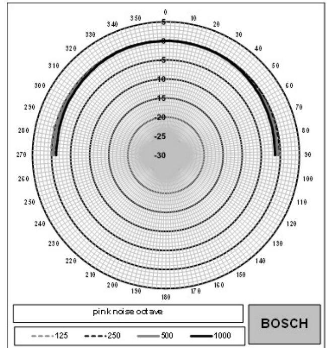
Fig. 2: Polar diagram LC1-PC30G6-6-IN low frequency part (frequency in Hz)
