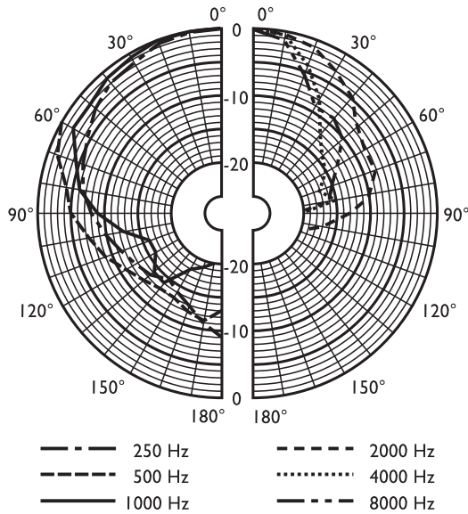
Figure 2.3: Polar diagram
