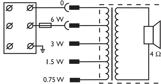
Figure 2.1: Circuit diagram
