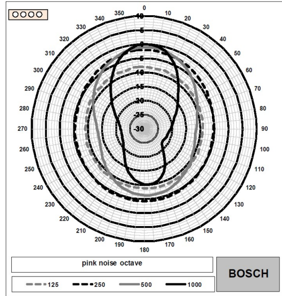
Fig. 6: Polar diagram LA2-UM40-LZD-IN (vertical measured with pink noise)
