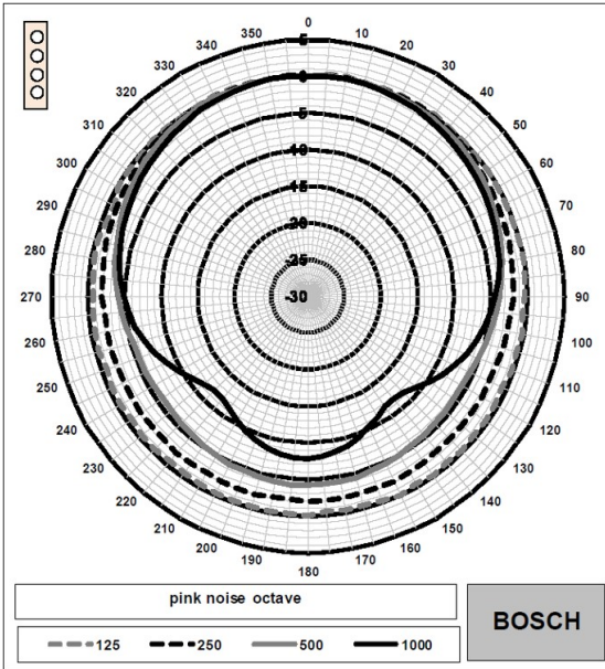
Fig. 4: Polar diagram LA2-UM40-LZD-IN (horizontal measured with pink noise)
