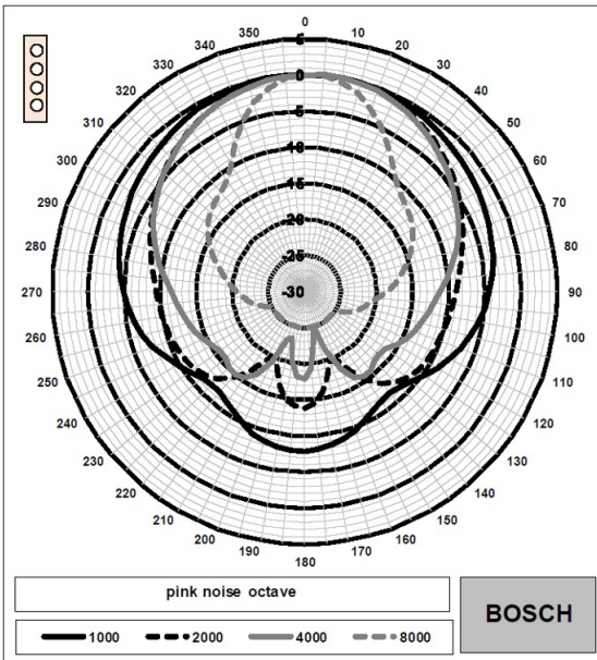
Fig. 5: Polar diagram LA2-UM40-LZD-IN (horizontal measured with pink noise)
