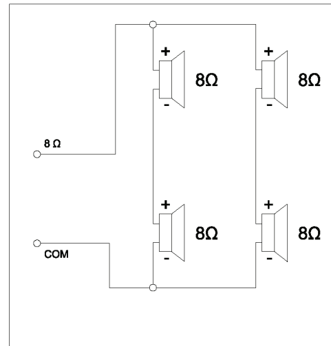
Fig. 2: Circuit diagram LA2-UM40-LZD-IN
