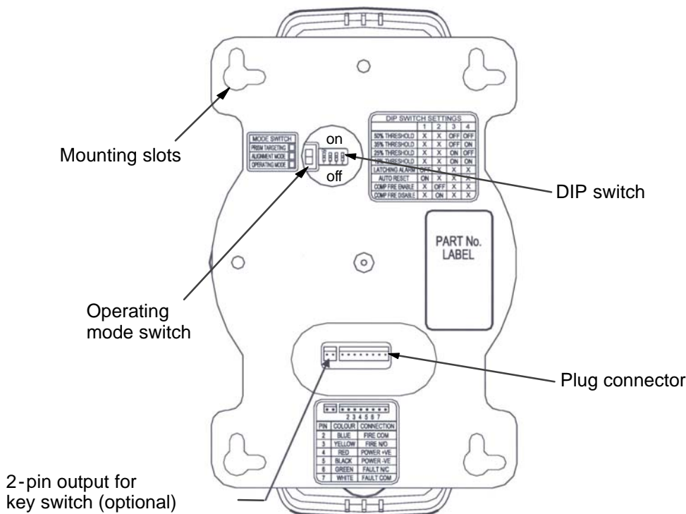
Fig. 2.: Reverse side of detector with plug connector, operating mode switch and DIP switch
