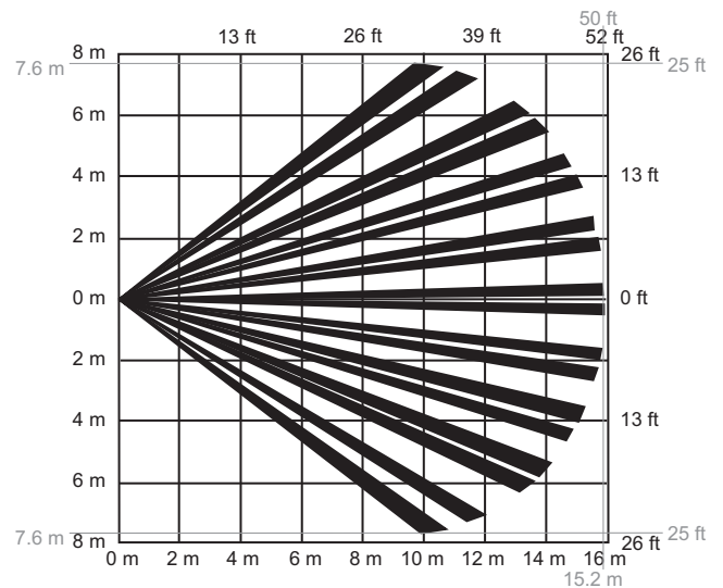
Top View: 30.4 m x 15.2 m (99.7 ft x 50 ft)
