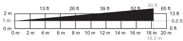
Side View: 3 m x 18.2 m (6.6 ft x 60 ft)
