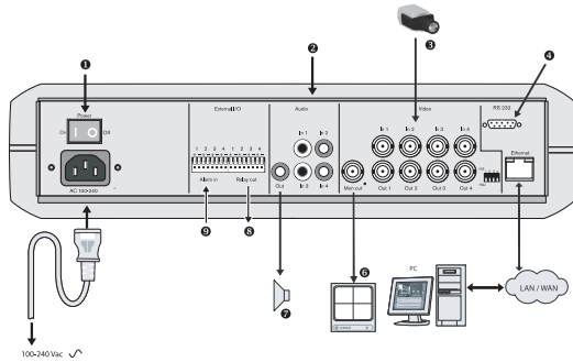
Connections on backside of DVR4C
