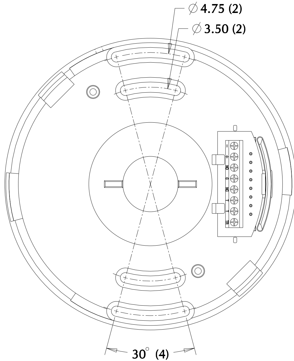
DS9360 CEILING MOUNT MOTION DETECTOR MOUNTING PATTERN AND WIRING LOCATIONS
