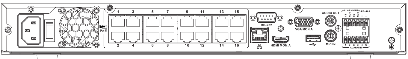
Fig. 2: Painel traseiro do DIVAR 3000 network (16 PoE)
