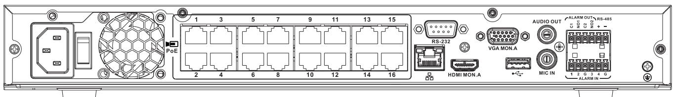
Fig. 2: DIVAR 3000 network, pannello posteriore (16 PoE)
