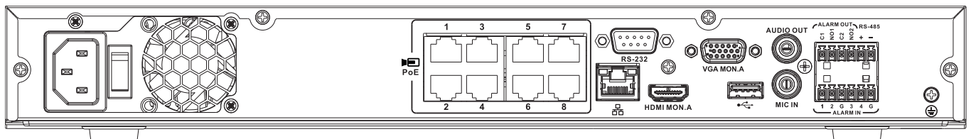
Fig. 2: DIVAR network 2000 (8 PoE), pannello posteriore
