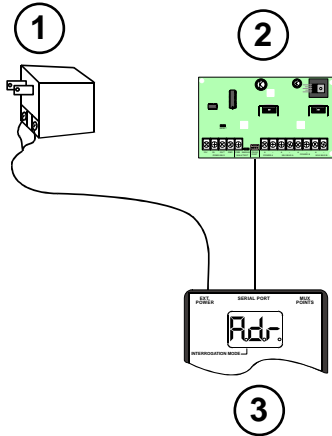
Figure 3: Wiring Diagram When Installing MUX Points With DIP Switches
