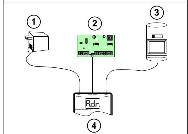
Figure 2: Wiring Diagram When Installing MUX Points Without DIP Switches
