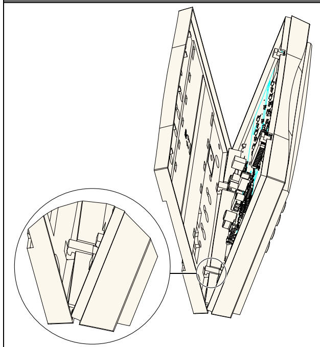
Figure 6: Reconnect Keypad to Base
