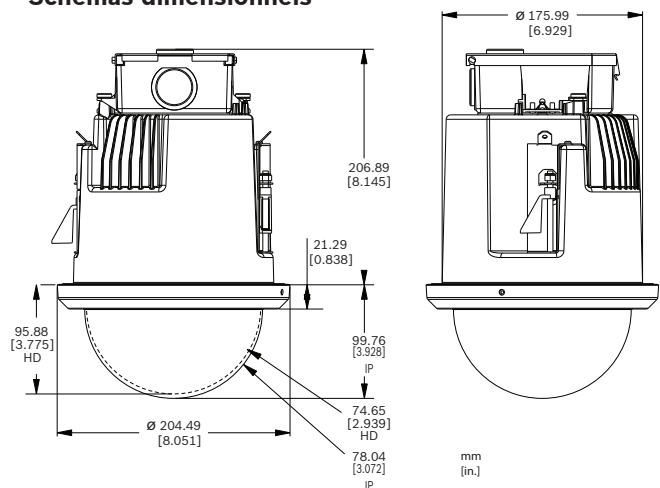
Fig. 1: AUTODOME 7000 series encastré
